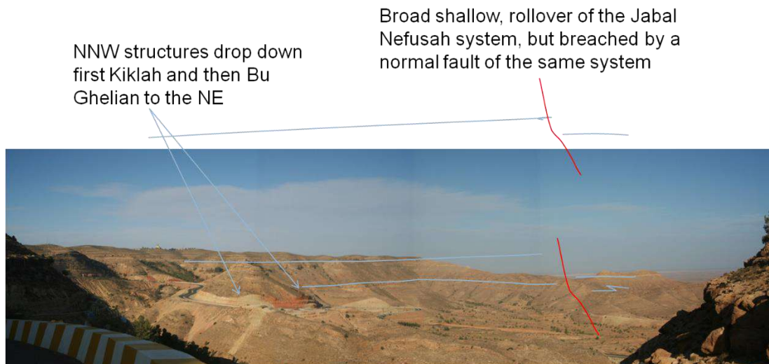
Figure (5): Nafusah Escarpment North of the Village of Abu Ghaylan. Kiklah Formation Displaced by Two Major Normal Faults of the Jabal Nafusah System and Forming a Broad, Low Amplitude Anticline Between Them.
