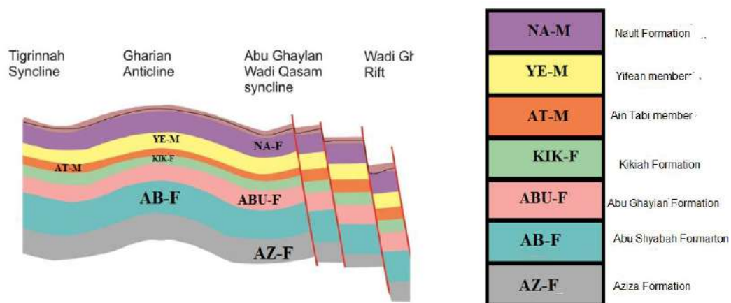
Figure (8): Differential Erosion and its Interplay with the Main Structures over Time.
